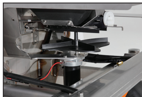
Spread dry materials up to 25-feet wide thanks to a high-torque electric spreader motor.
