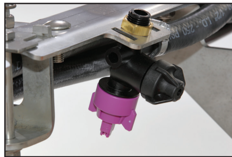
Replaceable nozzle design (with strainer) accommodates most standard tips, allowing you to install exactly the right tip for the job and conditions.
